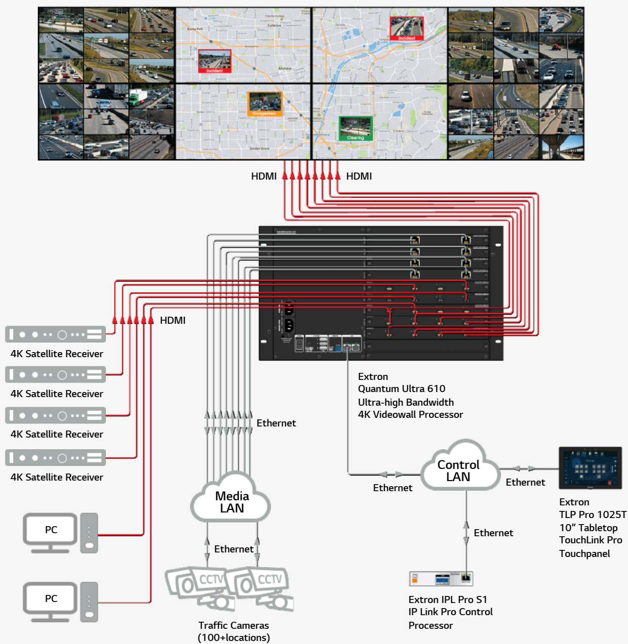
Figure 21 Major configuration of the Extron Quantum Ultra system
