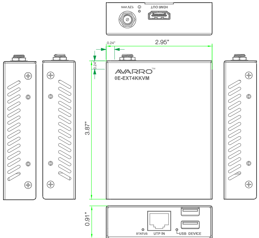
Receiver
