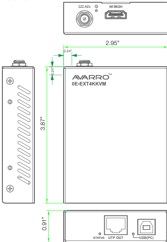
Transmitter
