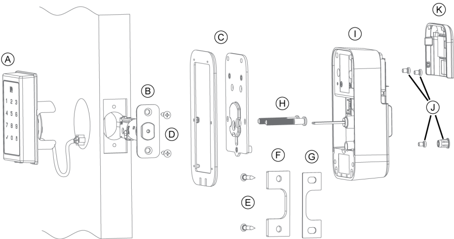
Figure 4: Smart lock installation overview
