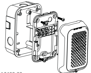
FIGURE 7. COMPACT SMBB
