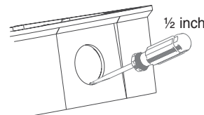
FIGURE 9 AND 10 . KNOCKOUT AND WIRE MOLD REMOVAL FOR SURFACE MOUNT BACK BOX
