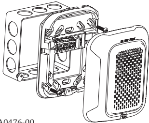
FIGURE 3. STANDARD DEVICE
