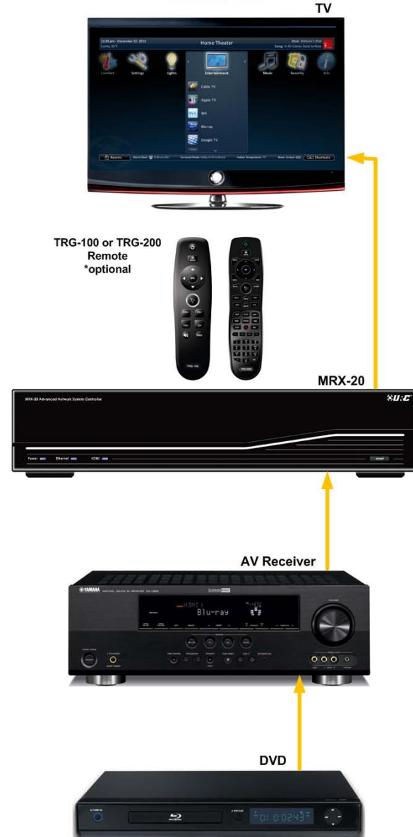
MRX-20 Application - Using With an AVR & TV
