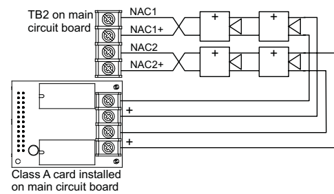
SA-CLA wiring
