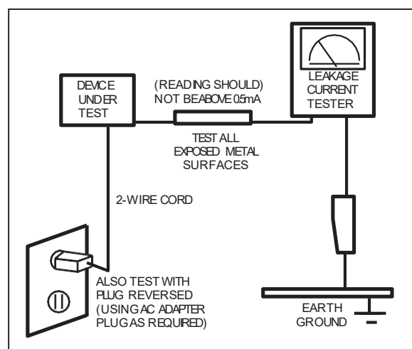
<Fig. 1-1 AC Leakage Test>
