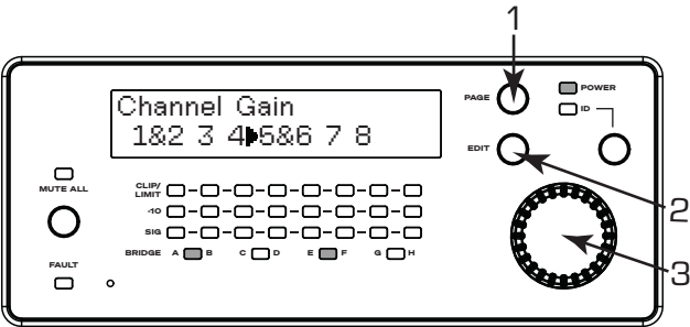
— Figure 17 — Gain Page - Channels 1&2, 5&6 Bridged
