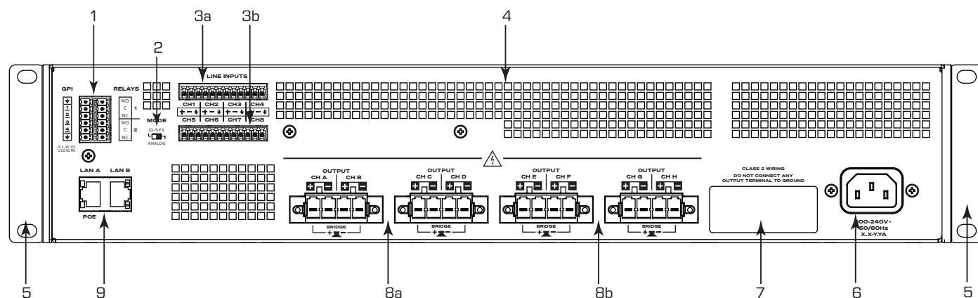
— Figure 1 — 8-Channel Model Shown
