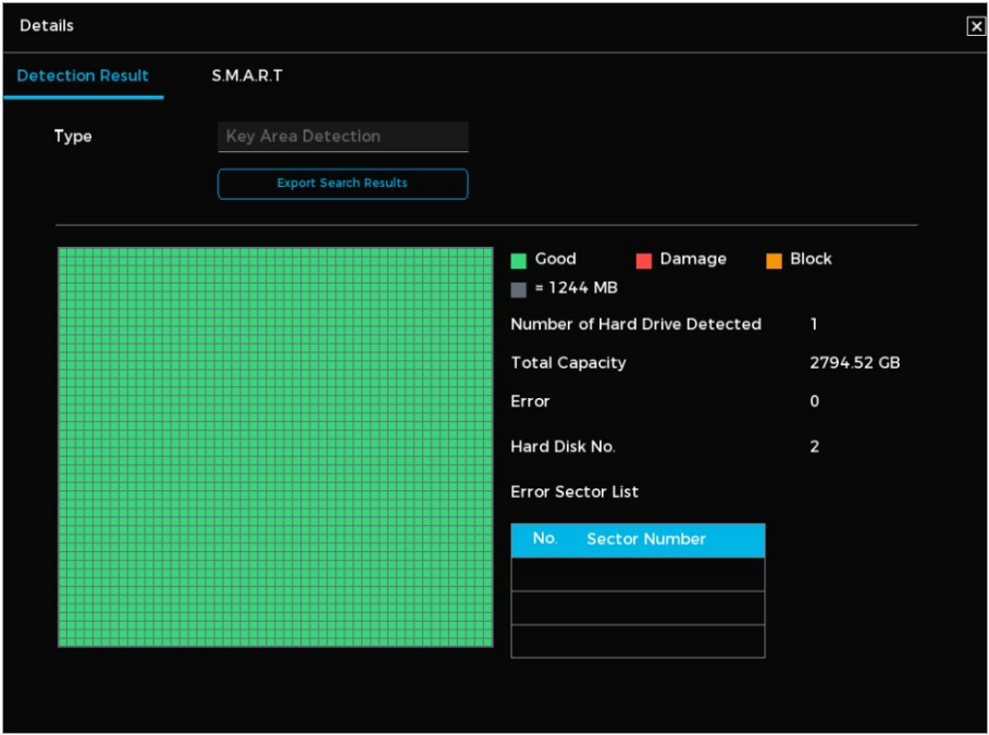
S.M.A.R.T. Report
