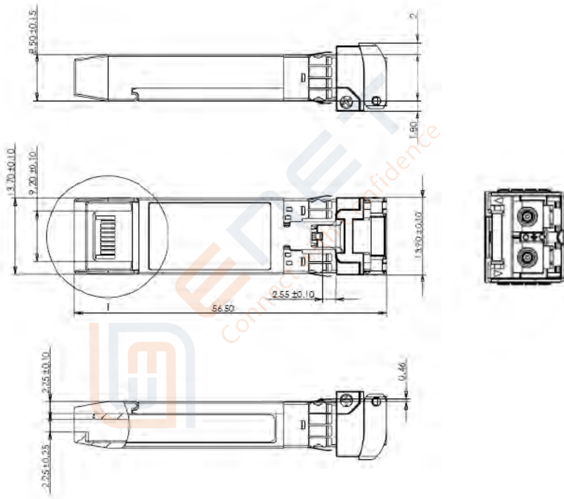
Figure 4. Mechanical Outline
