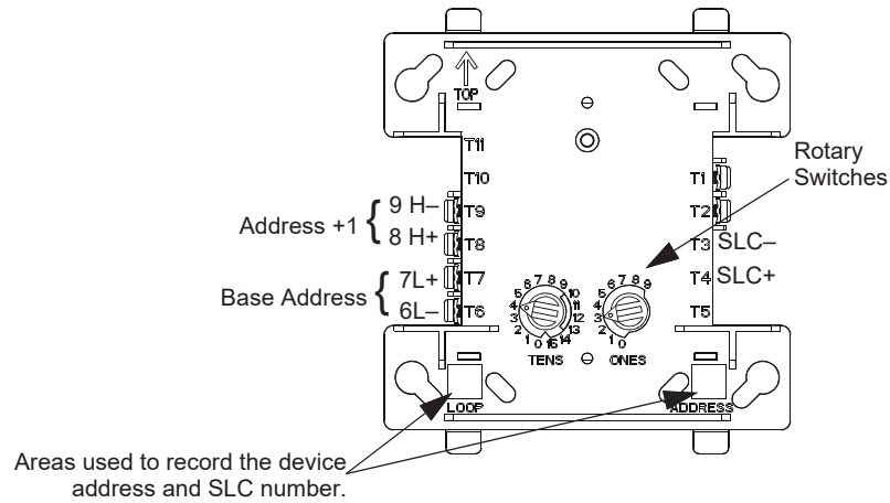
Figure 5.7 IDP-MONITOR-2 and SK-MONITOR-2 Dual Monitor Modules
