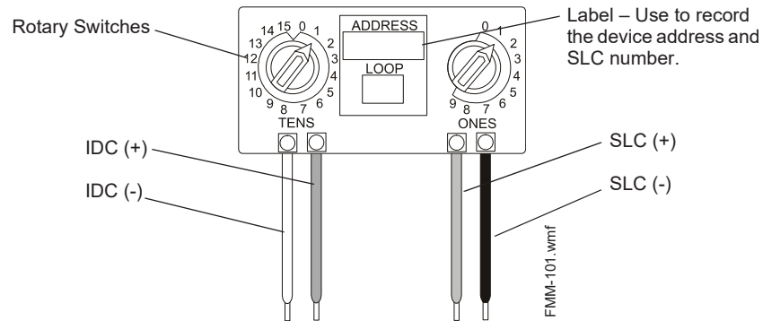
Figure 5.8 DP-MINIMON and SK-MINIMON Mini Monitor Modules
