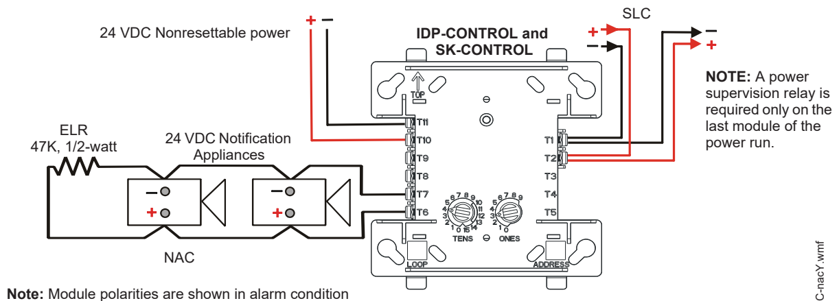
Figure 6.3 NFPA Class B Notification Appliance Circuit with IDP-CONTROL and SK-CONTROL
