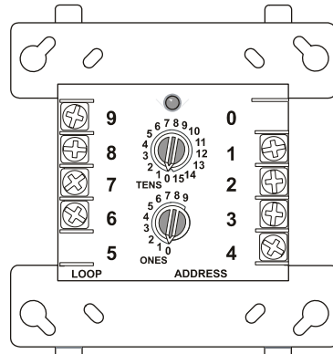
IDP-CONTROL and SK-CONTROL Legacy Version Module (Vertical Rotary Dial)
