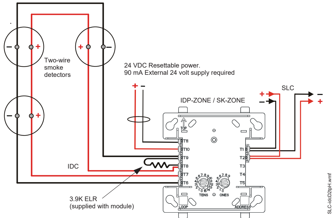
Figure 5.21 Typical Class A IDC Wiring with an IDP-ZONE and SK-ZONE
