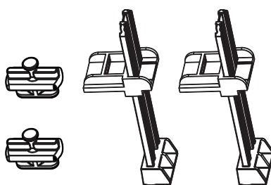
Forward Ratchet and Keyhole Post Clips (4) AC1051-RCKH-4
