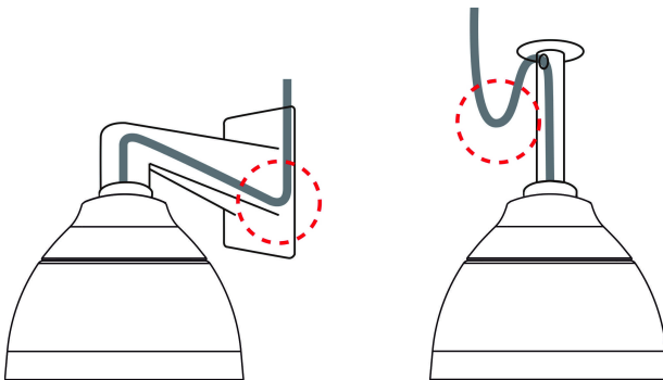
U-Shaped Cable Installation
