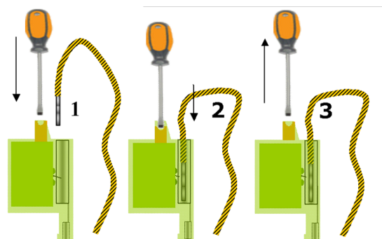
Connecting a Wire to a Spring Clamp
