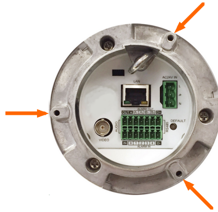
Pendant Cap Screw Holes on Camera (IR PTZ Models)
