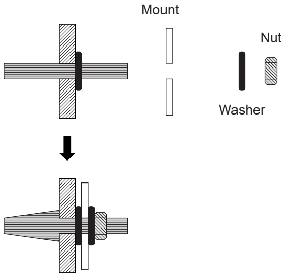
Figure 3: Attach the wall mount
