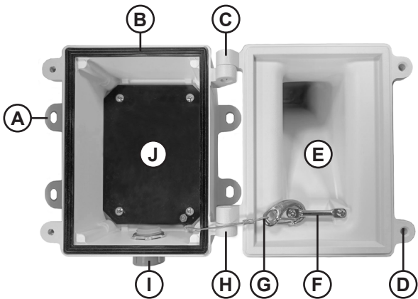
Figure 1: Wall mount assembly
