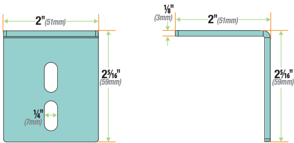
Mounting Bracket Dimensions
