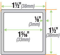
Frame Tube Dimensions
