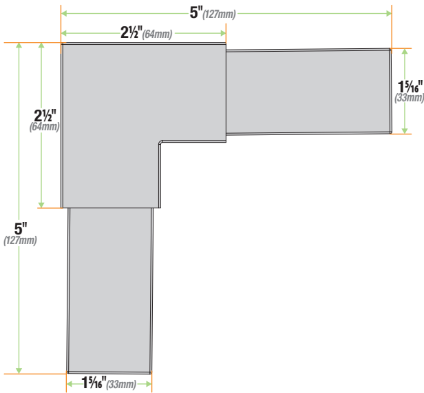
Connector Dimensions
