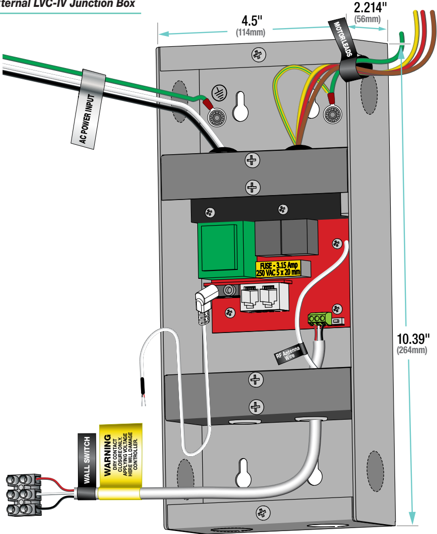
External LVC-IV Junction Box
