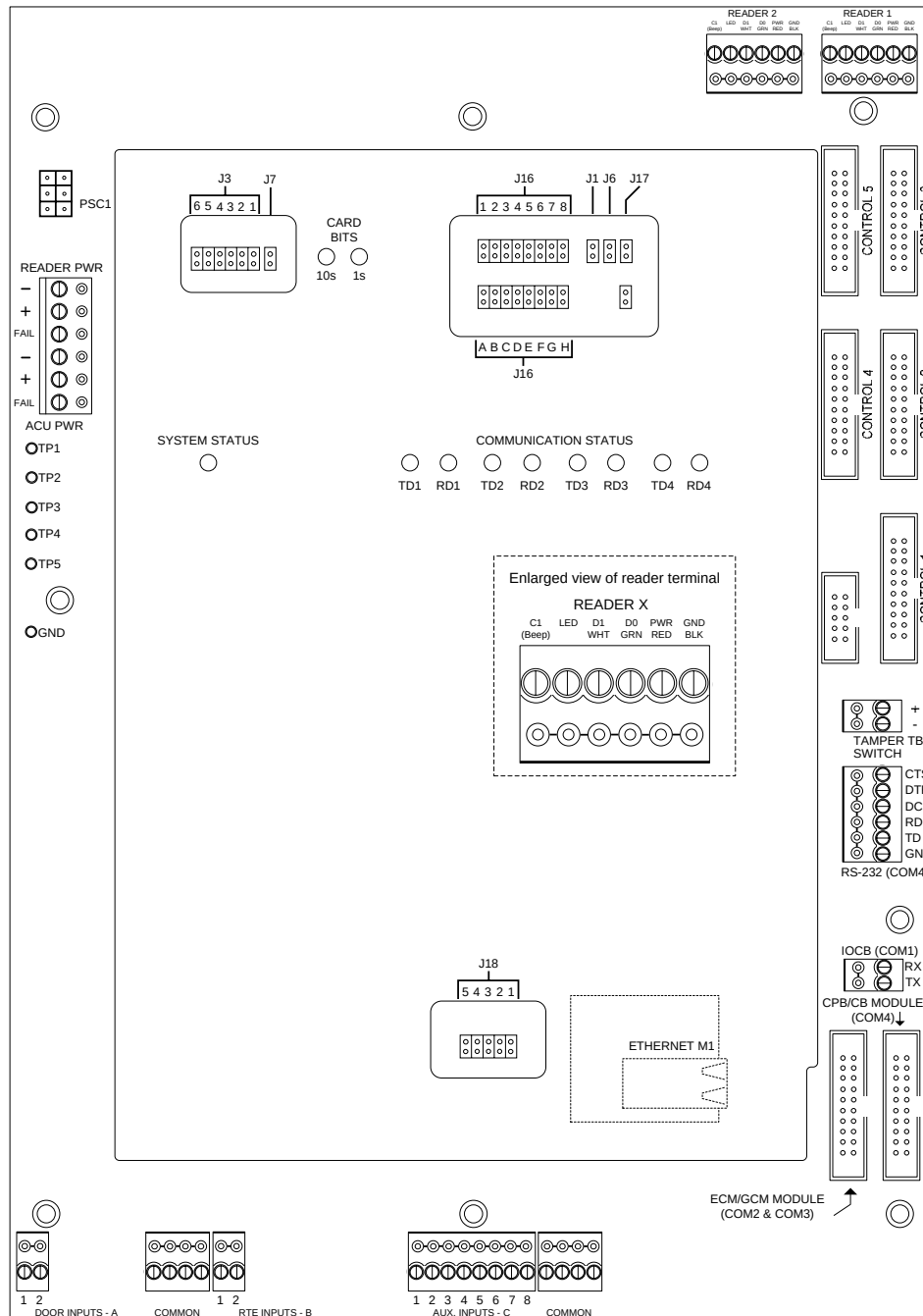
Figure 131 – CA250B Control Board
