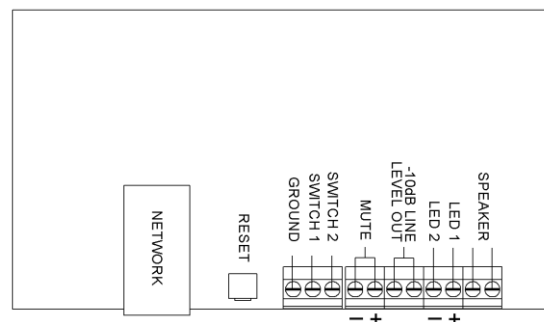
Figure 2. Connections
