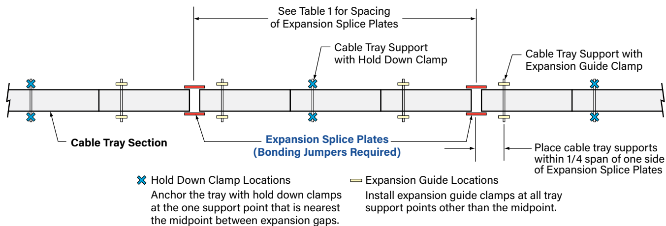
Figure 2a Cable Tray Expansion Connector Installation Locations
