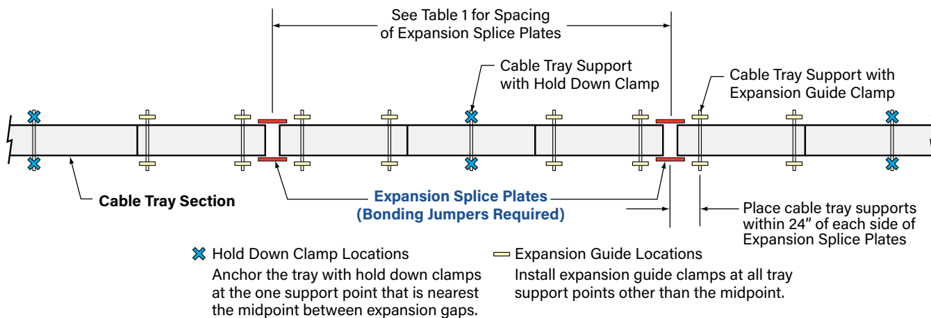
Figure 2b Expansion Connector Installation Locations
