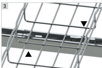
3 Add an additional FS41 on the opposite side of the channel support for secure installation.
