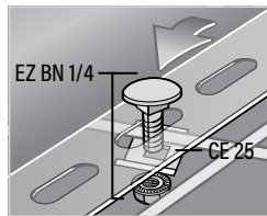
COT 54/COT 105 MOUNTING
