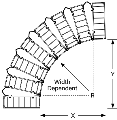
HORIZONTAL BEND 90 DEGREE (TIGHT AS POSSIBLE)
