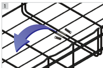
1 Remove outer mask of protective tubing (painted over) exposing the conductive tape at each end of the tray.
