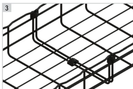
3 Add another SWK to the bottom section over the conductive tape for proper grounding.
