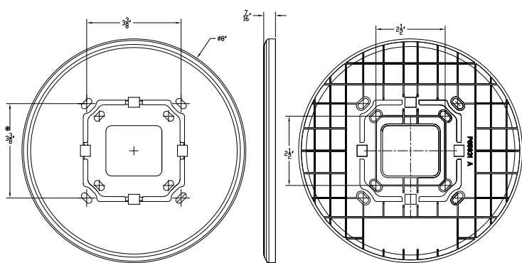
Figure 3. ELTP-UNI-C
