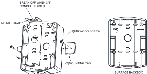
Figure 6: ELSPKBB Surface Back Box
