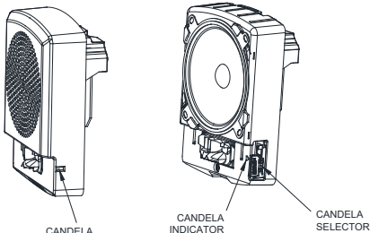
Figure 3B: Candela Setting Set from rear. Factory Setting is 15cd.
