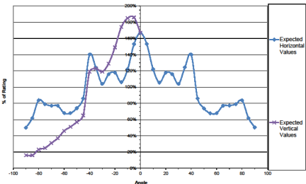
Figure 4: Light Distribution
