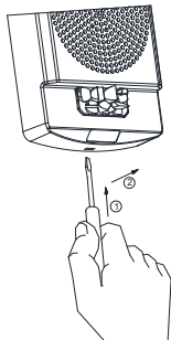
Figure 7: Grille Removal **
