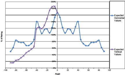
Figure 6: Strobe Light Distribution
