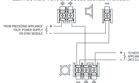
Figure 1A: One circuit. ELMTSC Multi-Tone and Strobe activate in unison.
