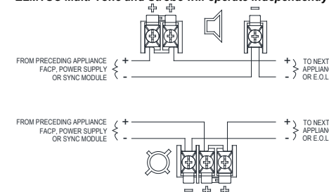
Figure 1B: Two Circuits (Multi-Tone may be Coded) ELMTSC Multi-Tone and Strobe will operate independently
