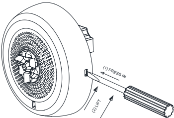
Figure 7: Grille Removal **
