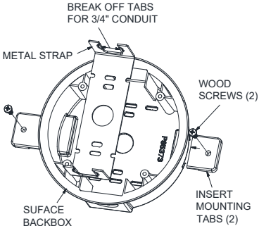
Figure 8: Surface Back Box – LSPKBB-C
