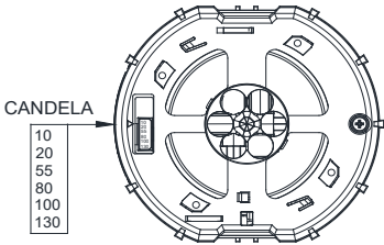
Figure 5: Candela
