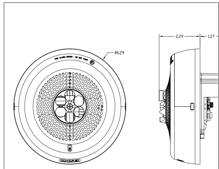
Figure 2. Ceiling chime strobe
