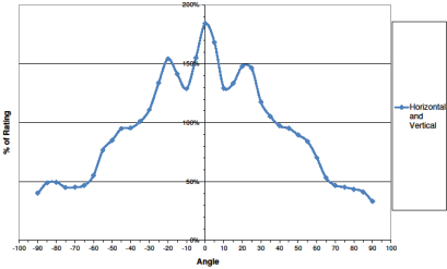
Figure 4: Light Distribution
