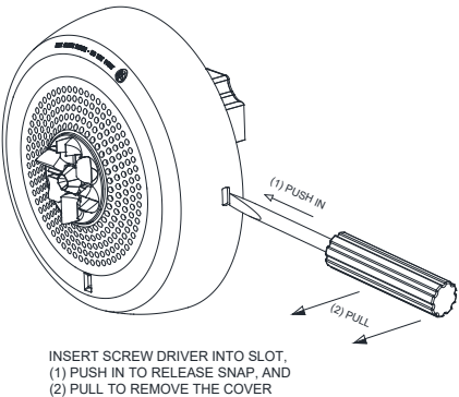
Figure 5: Grille Removal **
