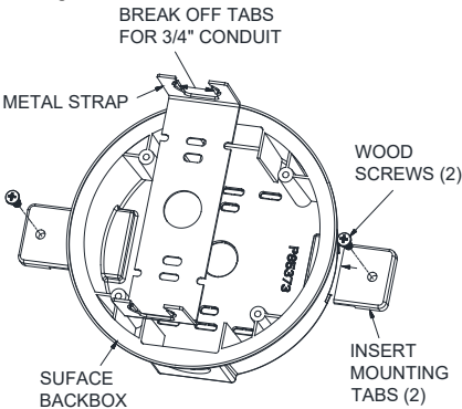
Figure 6: Surface Back Box – LSPKBB-C
