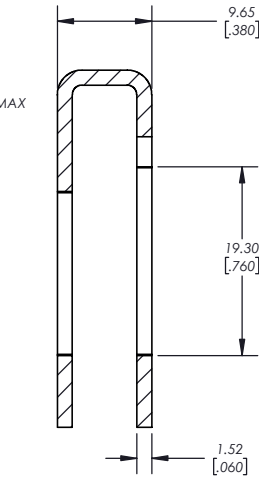
SECTION Z-Z
