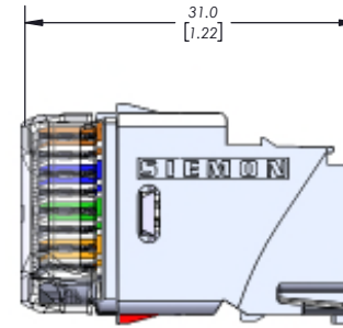
PANEL OUTLET U(XX)-P00N(X)
