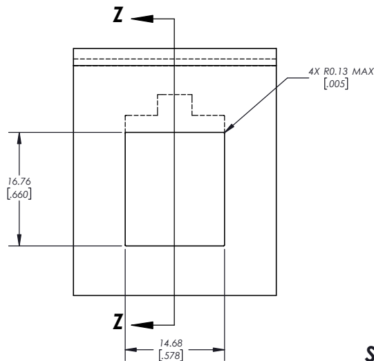
KEYSTONE PANEL CUTOUT & MOUNTING INFORMATION
