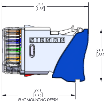
HYBRID OUTLET U(XX)-H(XX)(X)(X)
