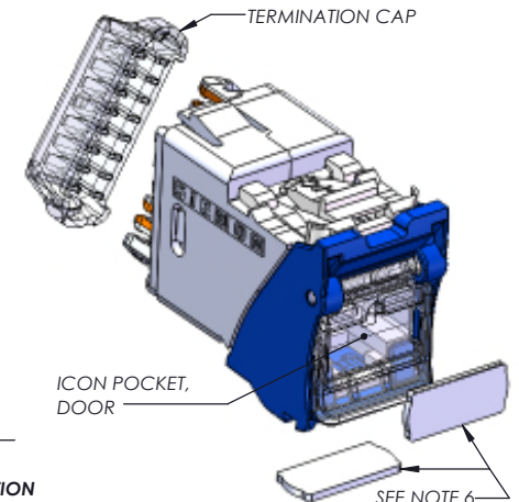
HYBRID OUTLET W/ DOOR U(X)-H(XX)D(X)
