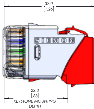
KEYSTONE OUTLET U(XX)-K(XX)(X)(X)
