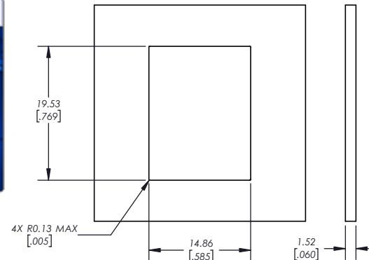
HYBRID PANEL CUTOUT & MOUNTING INFORMATION
