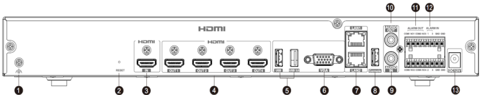
Rear panel
