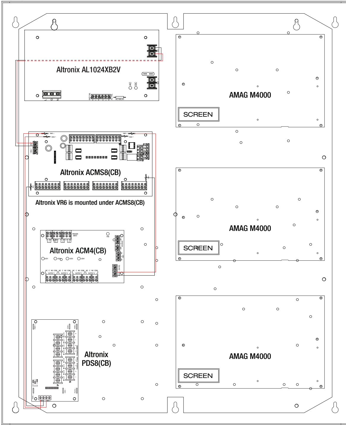
Fig. 5 - T2AGK712S(D)V Configuration
