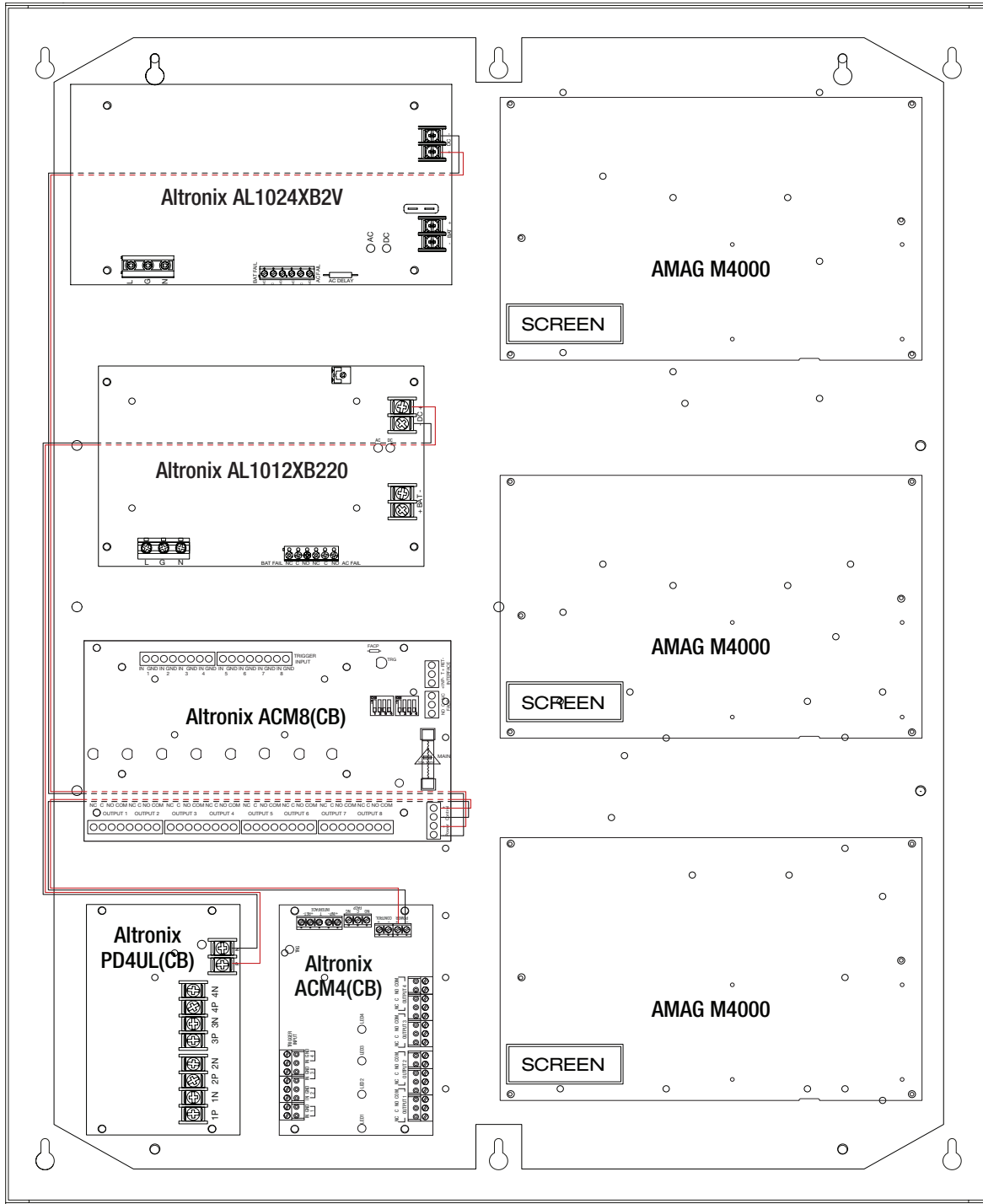
Fig. 6 - T2AGK7512(D)V Configuration
