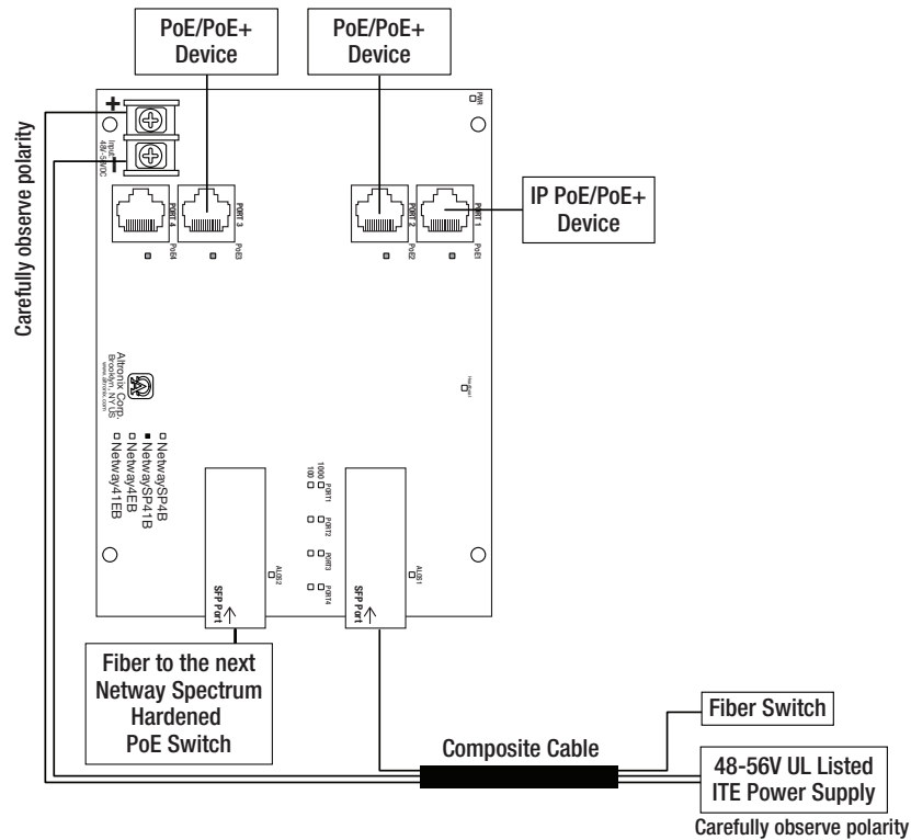
Fig. 3 - NetWaySP41WPN – Typical Application with Composite Cable
