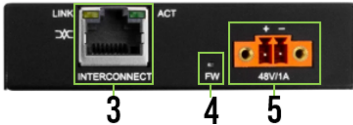
AC-EXUSB-3-HOST Rear Panel
