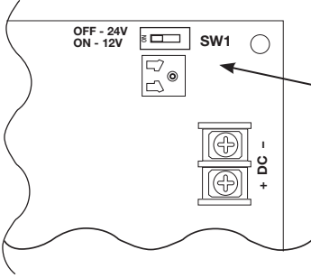
Fig. 1a - Maximal11 and Maximal33 Power Supply Board
