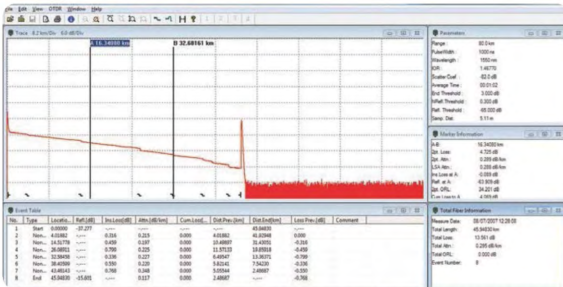
TraceViewer Software showing trace, event table, Parameters, Marker Information & Total Fiber Information.
