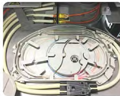
Macrobend easily visible in splice tray using 180XL
