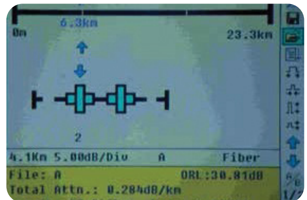
TraceViewer with expanded trace view highlighting the benefit of Launch Cables to examine Near & Far end connectors.
