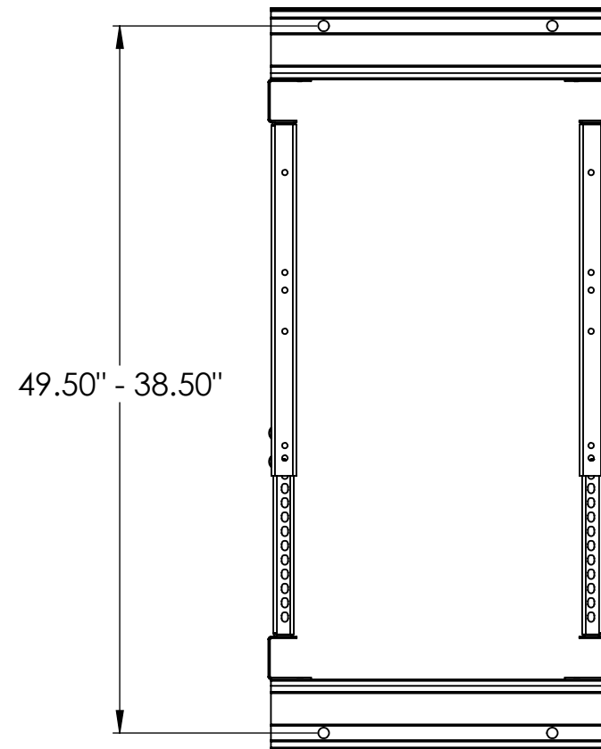
BOTTOM VIEW (MOUNTING HOLES- BRACKETS OUT)
