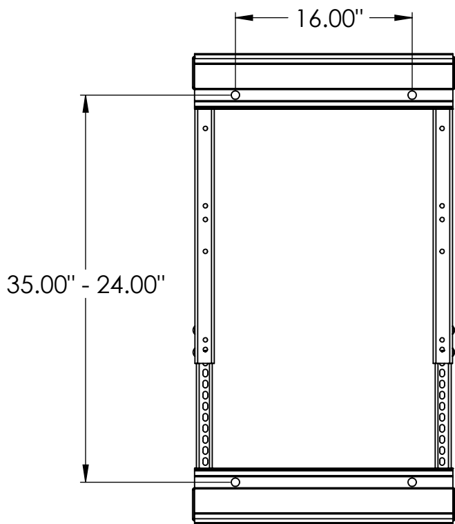
BOTTOM VIEW (MOUNTING HOLES- BRACKETS IN)
