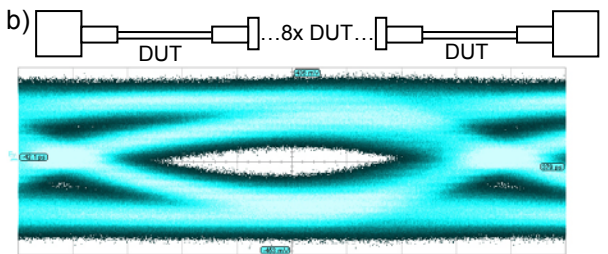
42.1 ps/div Figure 11
