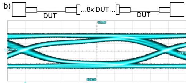
42.1 ps/div Figure 7
