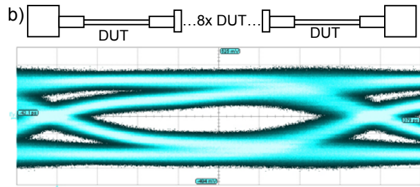
42.1 ps/div Figure 9
