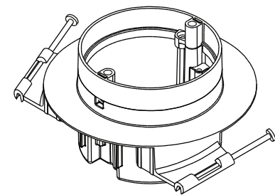
ISOMETRIC VIEW 1/4 SCALE
