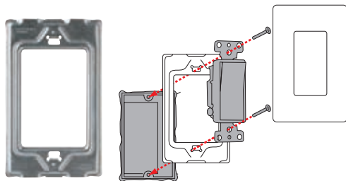
The P&S Decorator opening offers a metal subplate for commercial applications (SW26 series).
