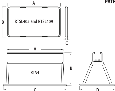
Sled snaps onto open base to allow for expansion and contraction without damaging roof surface
