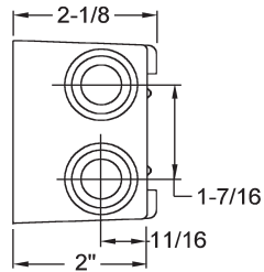
END VIEW TWO OUTLET
