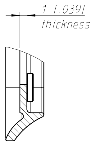
Detail X 3:1
