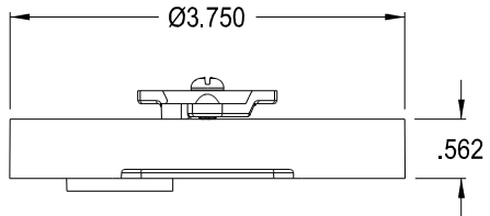
ASSEMBLY OF FSC405R W/ 5/8" WINGS
