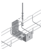
SF 100 CENTER HANGER SUPPORT CENTRAL DE SUSPENSION SOPORTE COLGANTE CENTRAL
