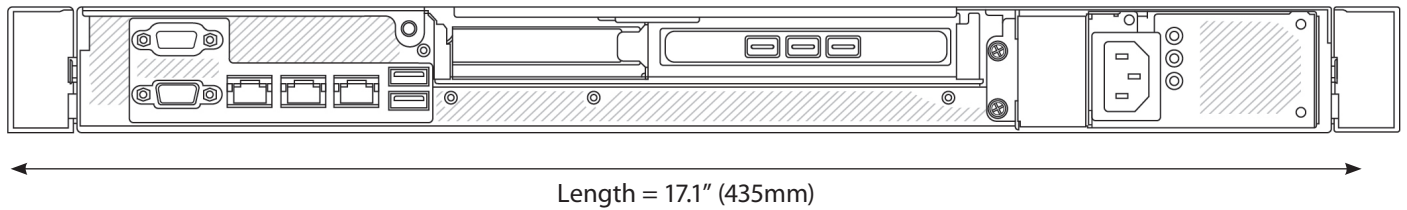
Rear View
