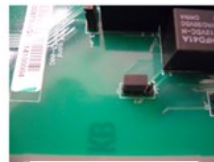
Figure B7 JP3 jumpered 1 to 2
