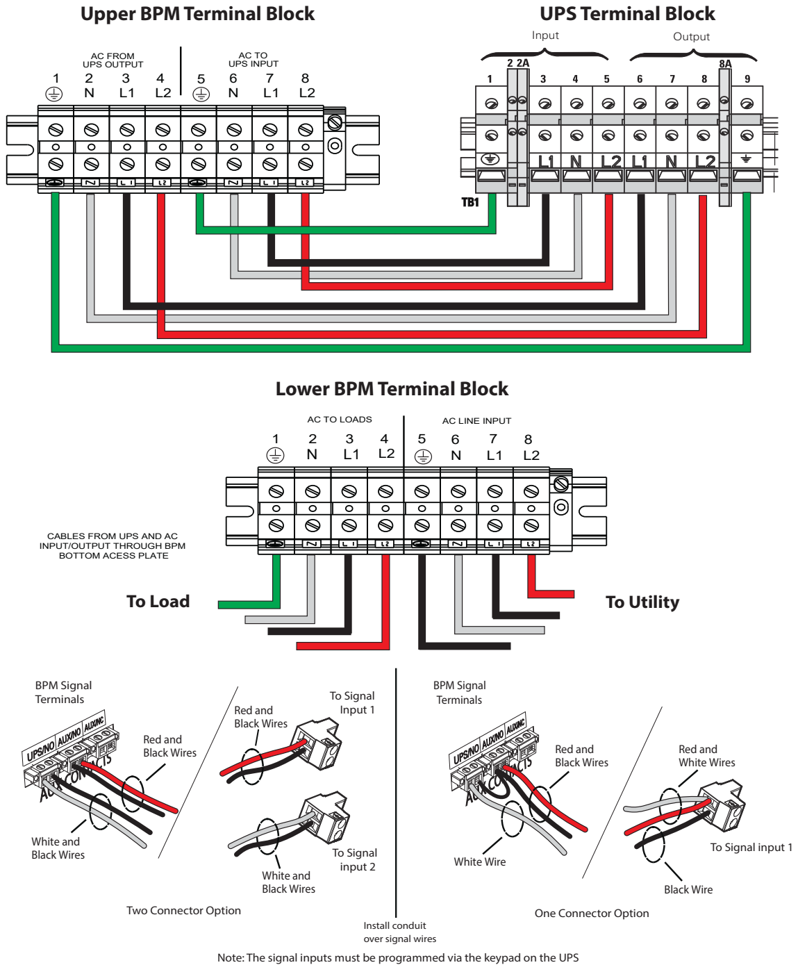
Figure 11. Eaton 9155 UPS to BPM Connection Diagram Using Signal Inputs
