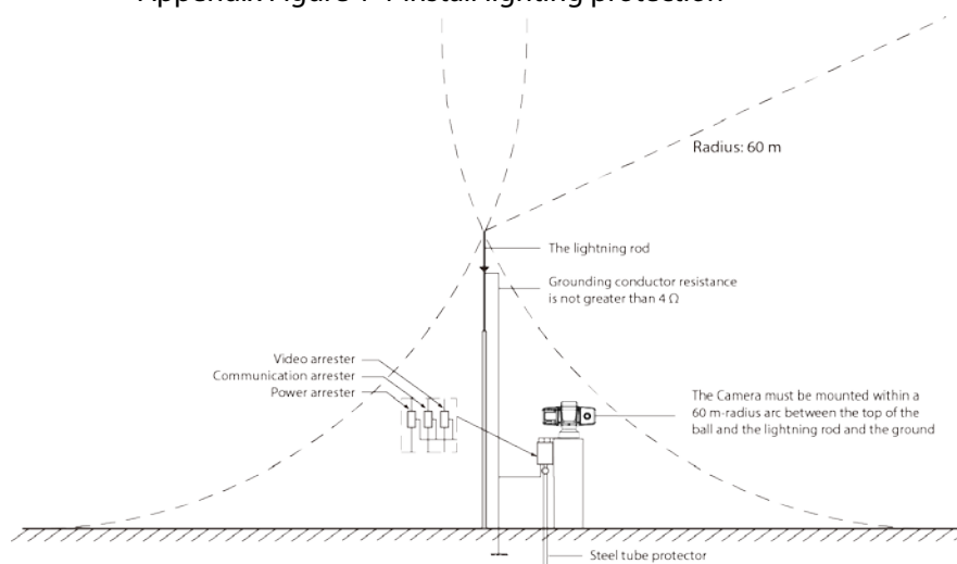
Appendix Figure 1-1 Install lightning protection
