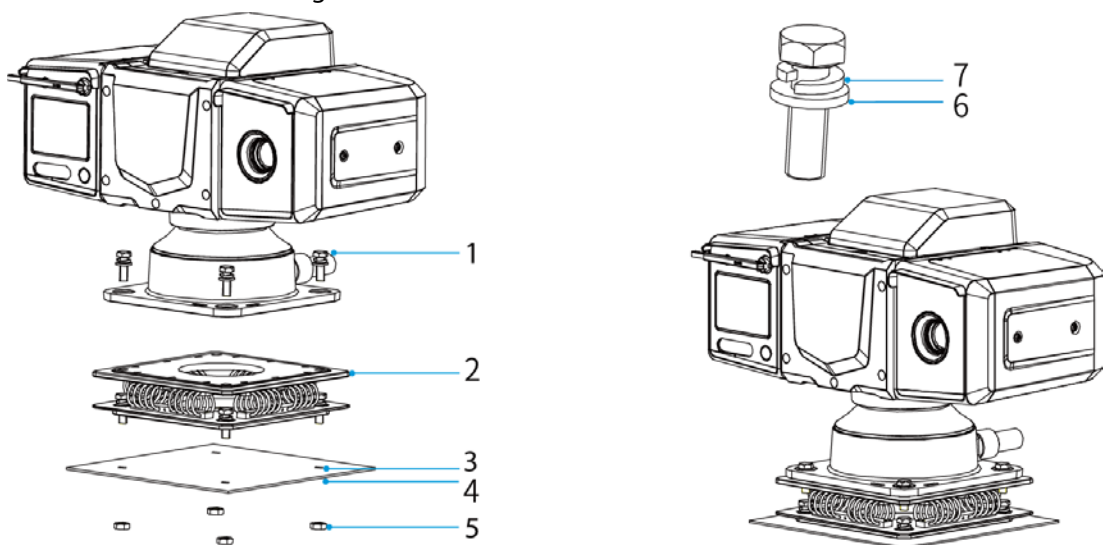
Figure 4-2 Fix camera onto a vehicle
