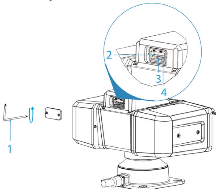
Figure 4-1 Install Micro SD card
