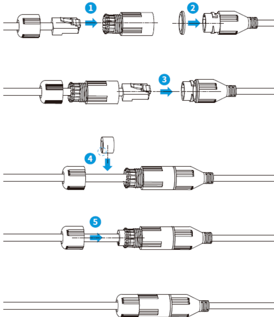
Figure 4-5 Install waterproof connector for network port
