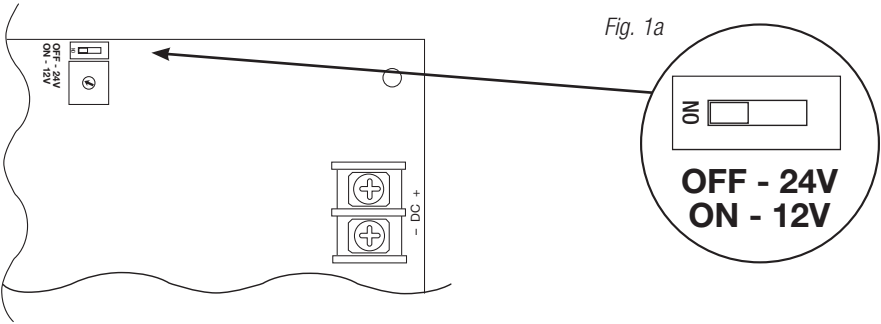
Fig. 1 - Maximal3DV Power Supply Board
