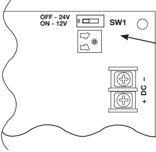
Fig. 1a - Maximal3D Power Supply Board
