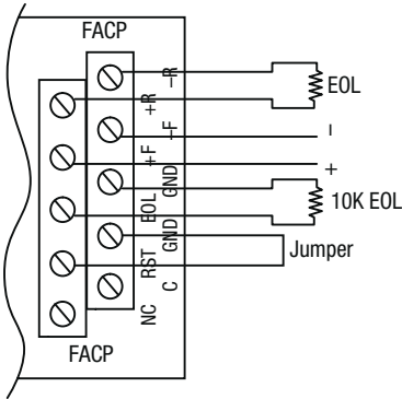
Fig. 13 - Normally Closed trigger input (Non-Latching).
