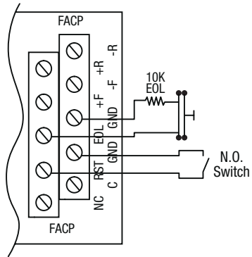
Fig. 16 - Normally Open trigger input (Latching).
